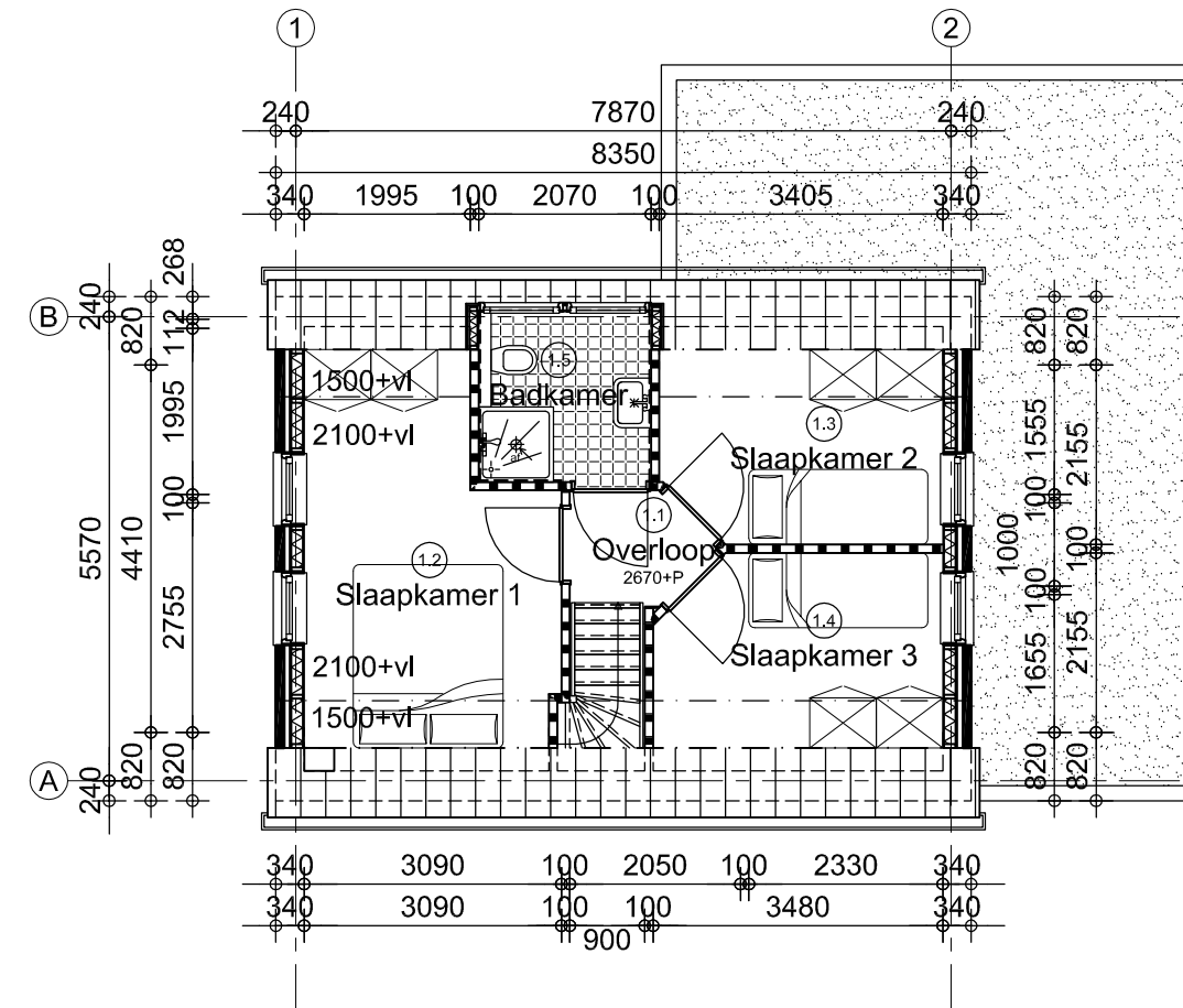
Verdieping variant 2
