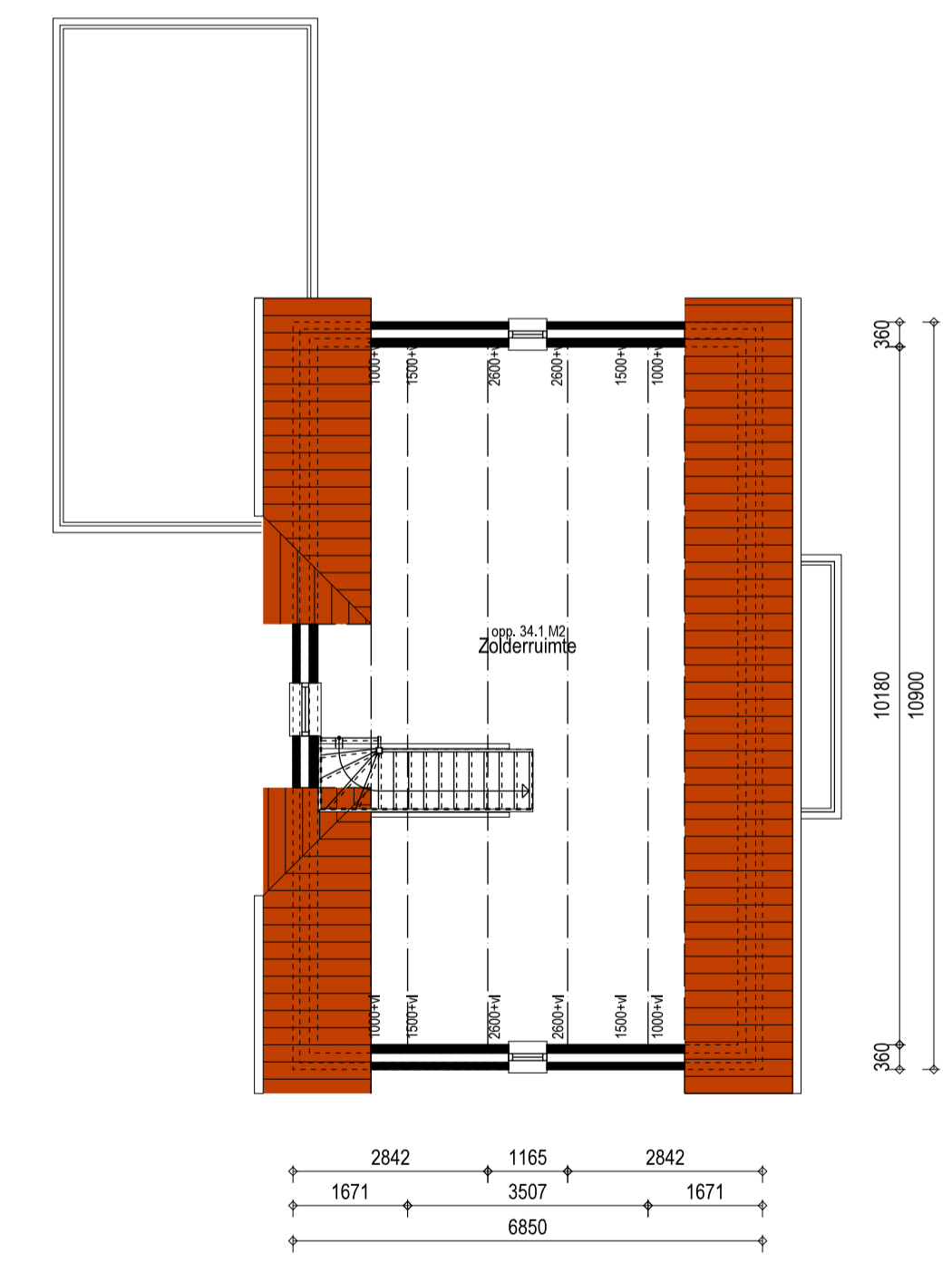
Zolder
