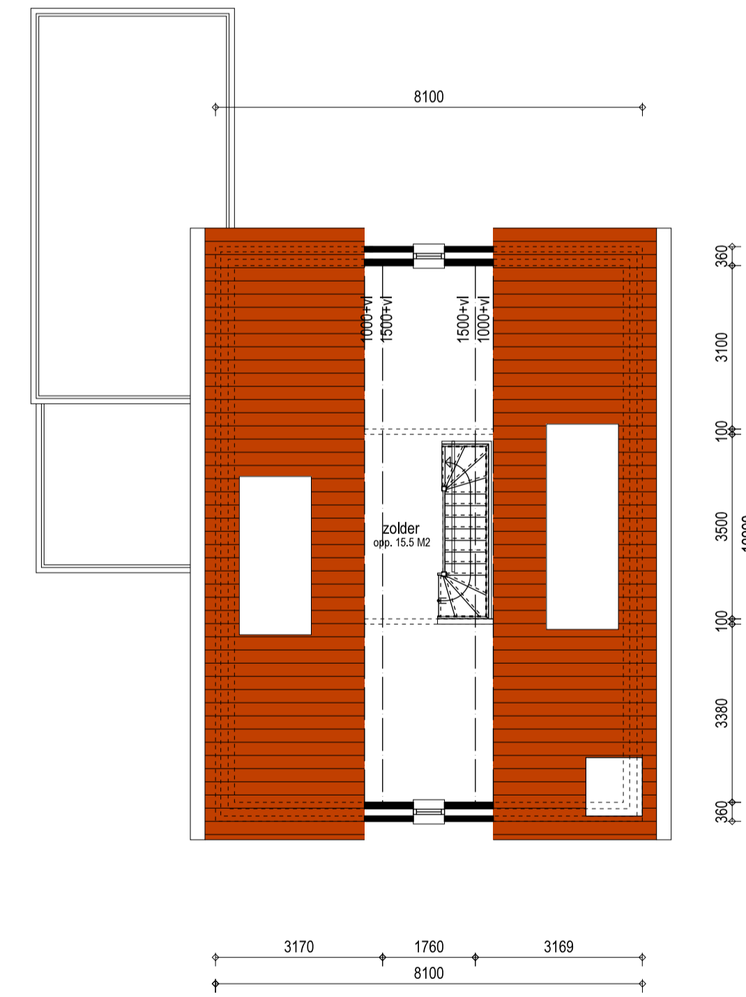
Zolder
