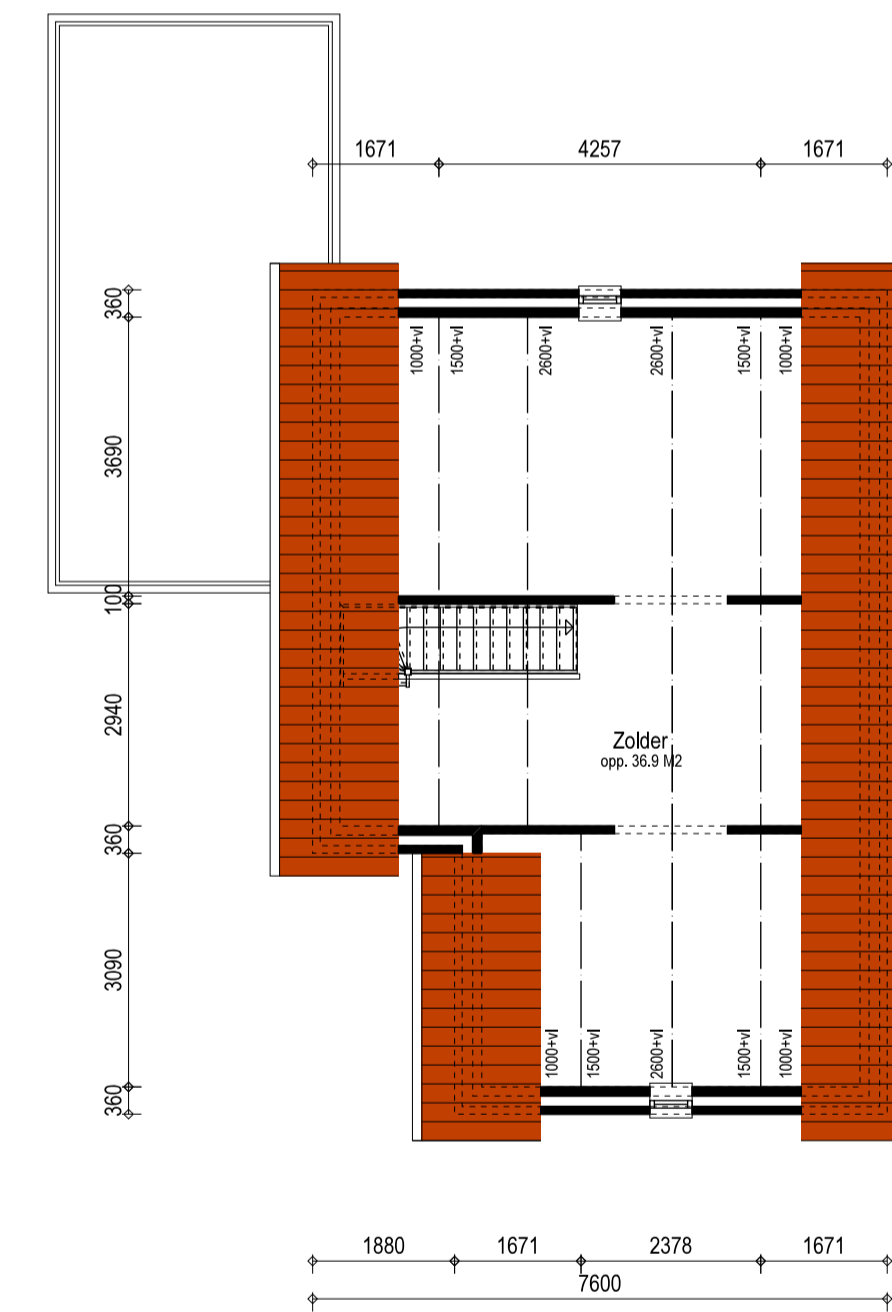
Zolder
